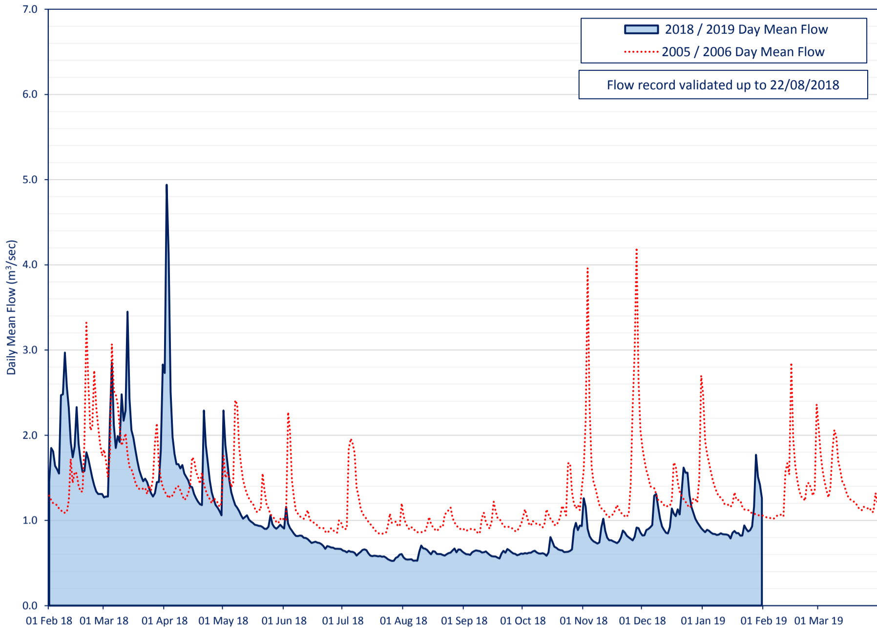
River Bure at Ingworth (12 Month Hydrograph)
