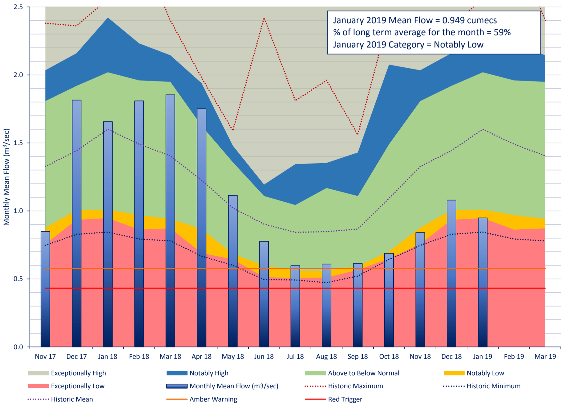
River Bure at Ingworth Flow Categorisation 1970-2012 (Featured Years - 2017 to 2018)
