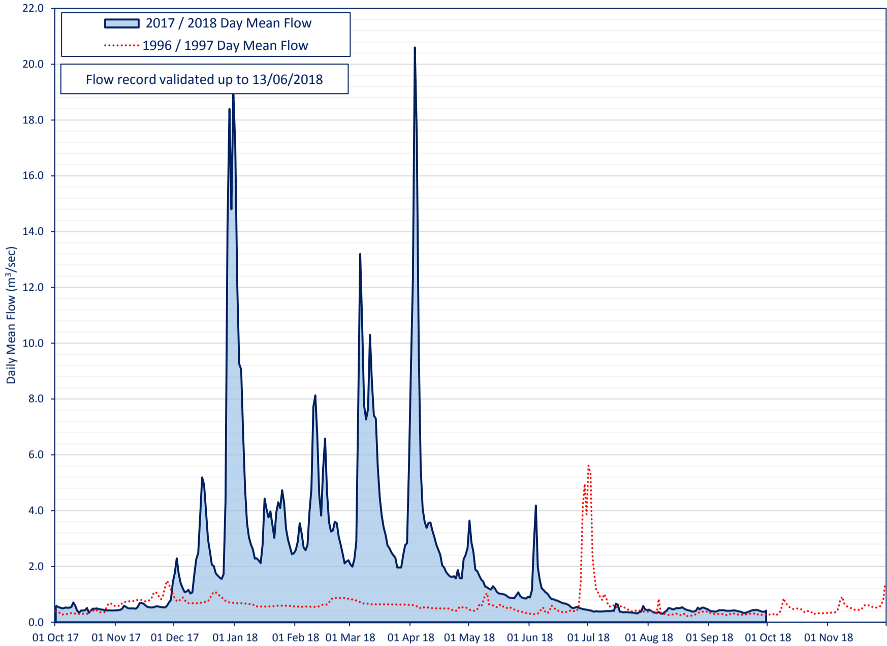
River Yare at Colney Flow Categorisation 1970-2012 (Featured Years - 2017 to 2018)
