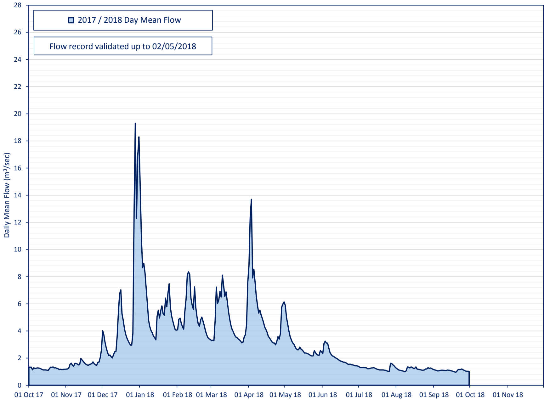
River Wensum at Swanton Morley Flow Categorisation 1969-2017 (Featured Years - 2017 to 2018)
