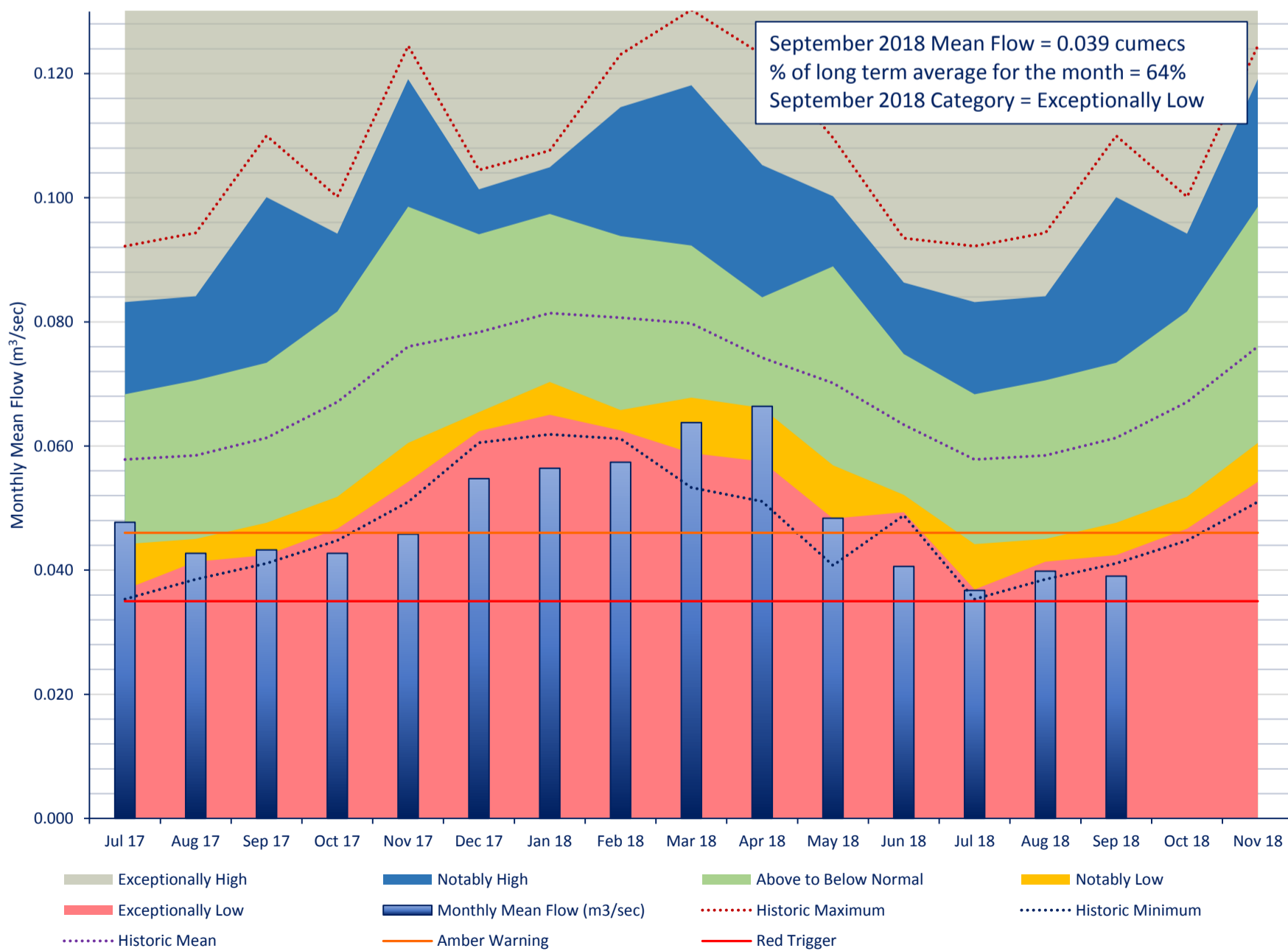
Black Ditch at Hollesley Flow Categorisation 1995-2016 (Featured Years - 2017 to 2018)
