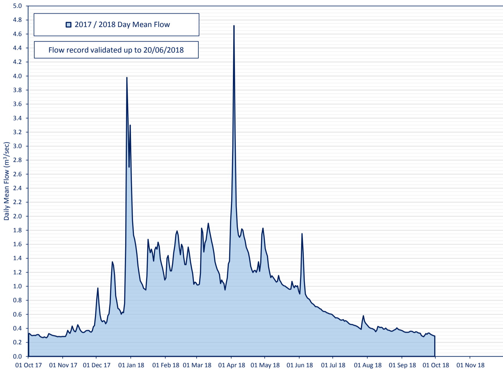
River Wensum at Fakenham Flow Categorisation 1970-2012 (Featured Years - 2017 to 2018)
