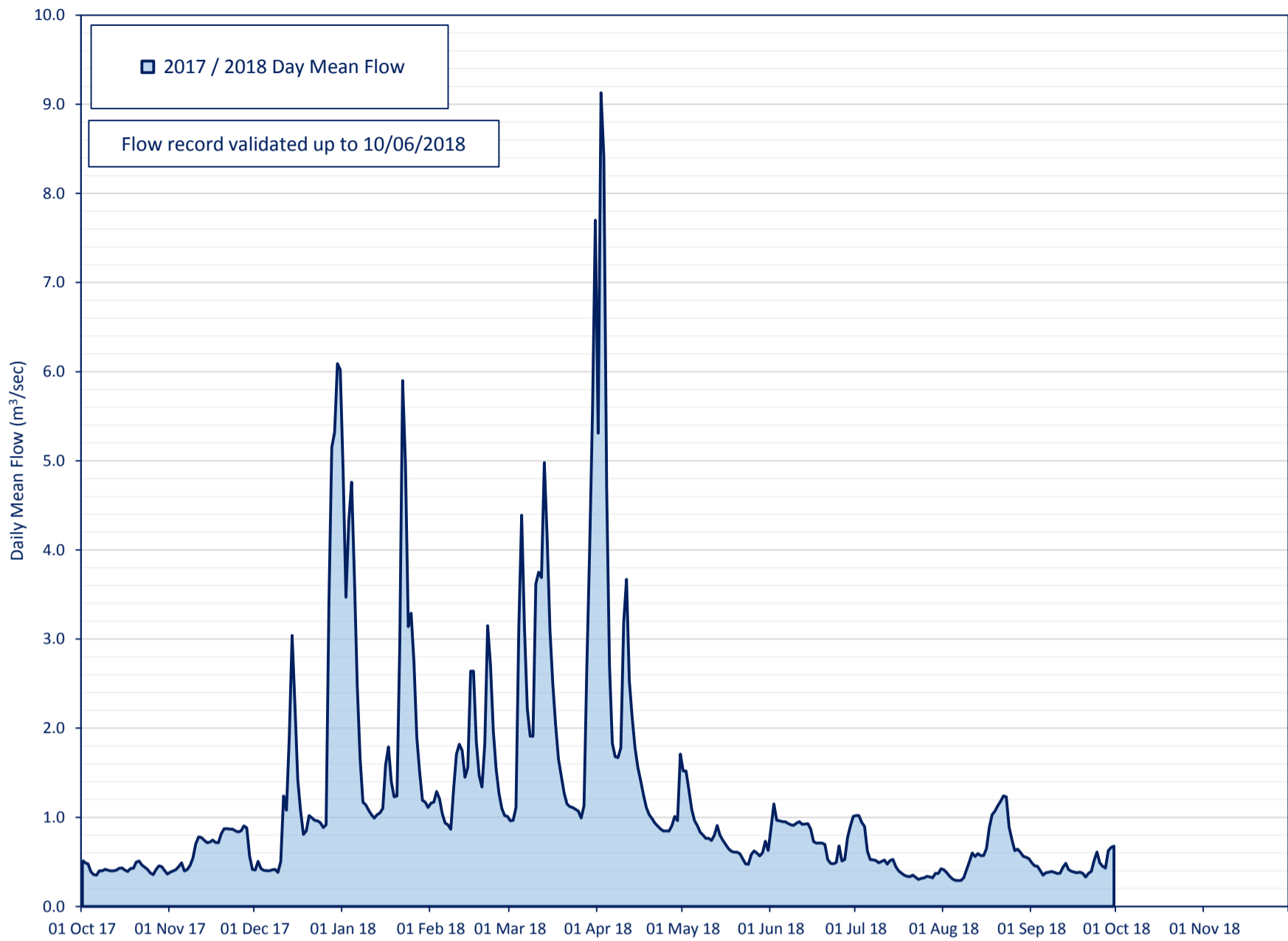
River Blackwater at Appleford Bridge Flow Categorisation 1970-2012 (Featured Years - 2017 to 2018)
