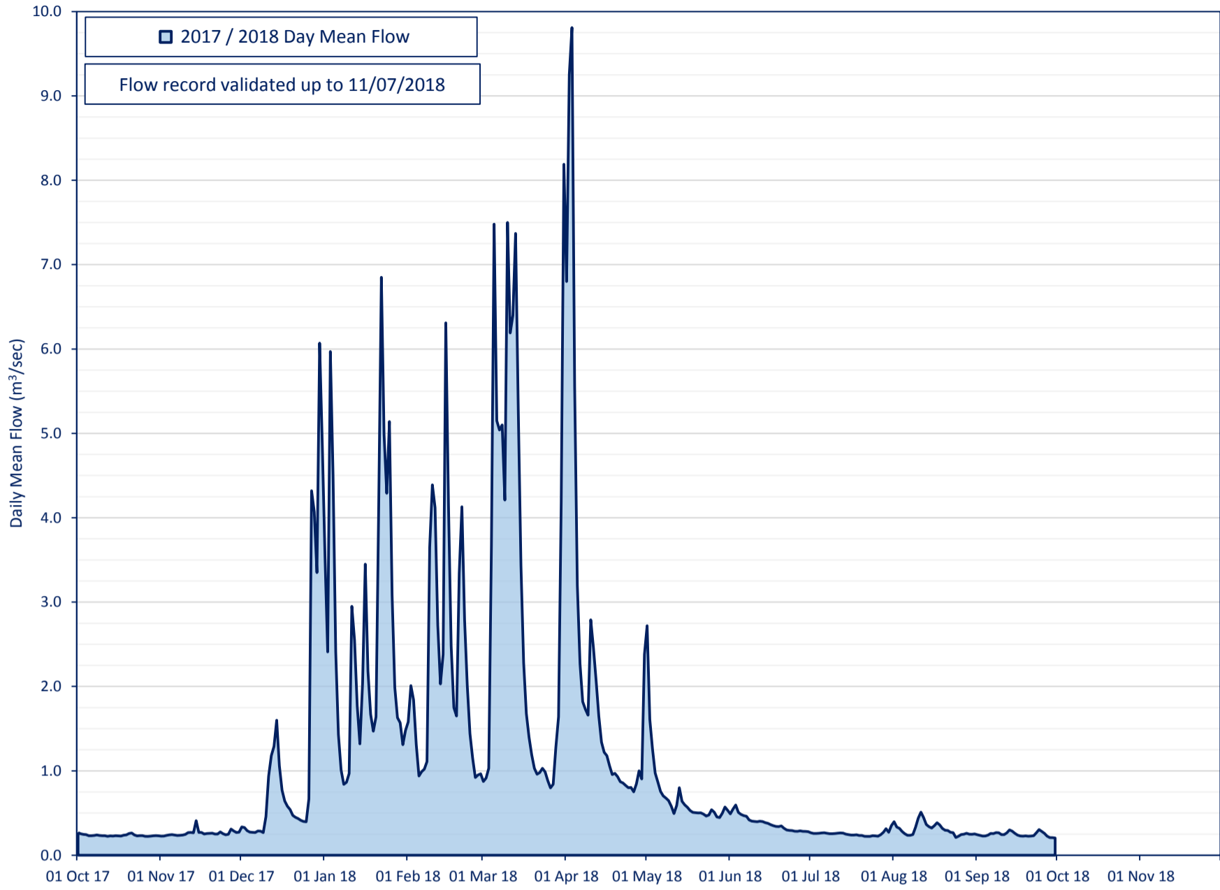
River Gipping at Bramford Flow Categorisation 1970-2012 (Featured Years - 2017 to 2018)
