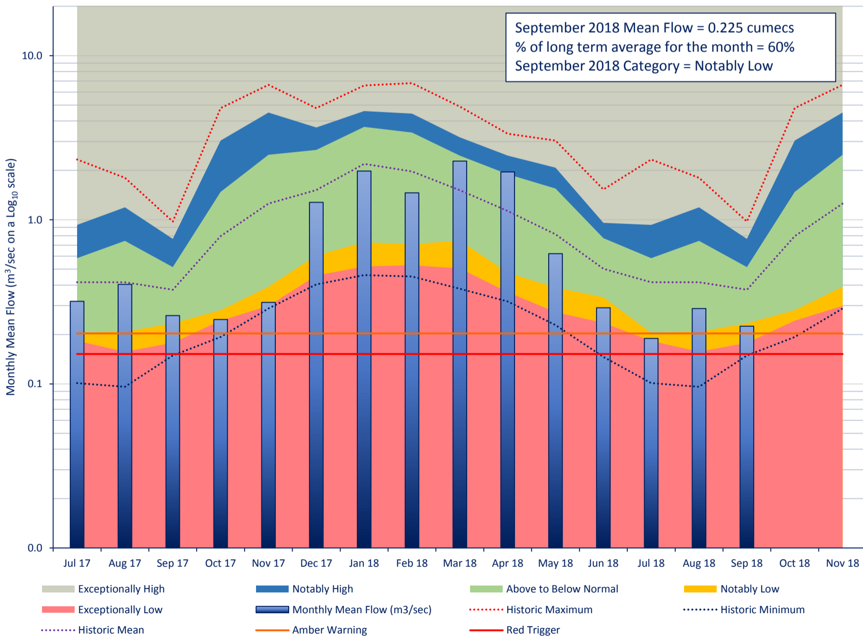
River Colne at Lexden Flow Categorisation 1970-2012 (Featured Years - 2017 to 2018)
